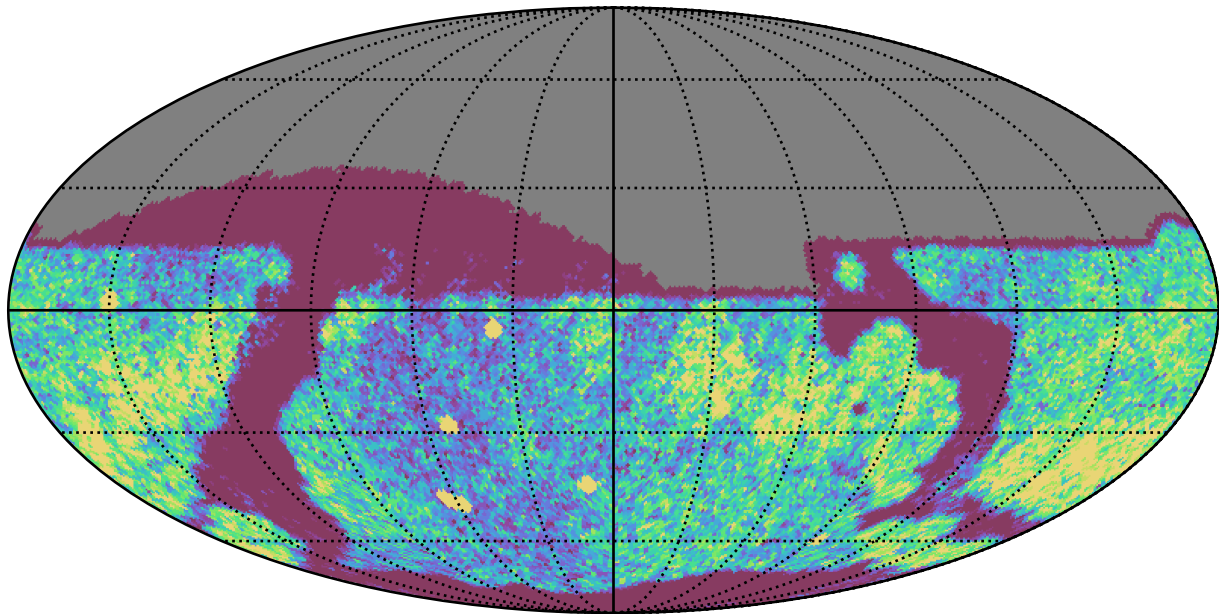
too_100_4v3.4_10yrs Yr 1 r band: NVisits
