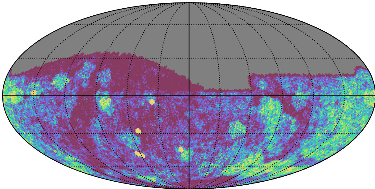
too_100_4v3.4_10yrs Yr 1 g band: NVisits
