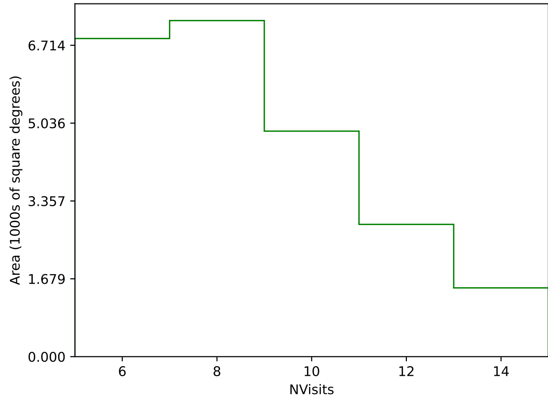
too_100_4v3.4_10yrs Yr 1 g band: NVisits
