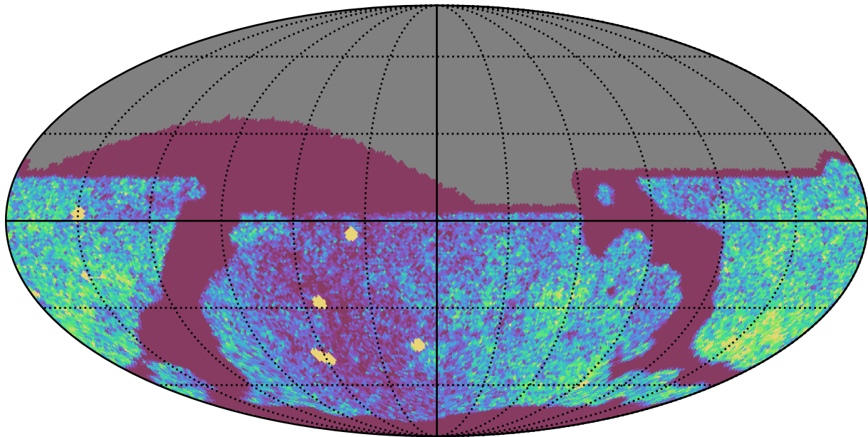
too_100_4v3.4_10yrs Yr 1 all bands: NVisits
