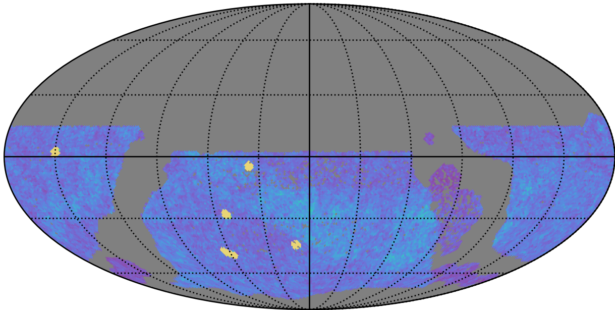
too_100_4v3.4_10yrs WFD z band: NVisits
