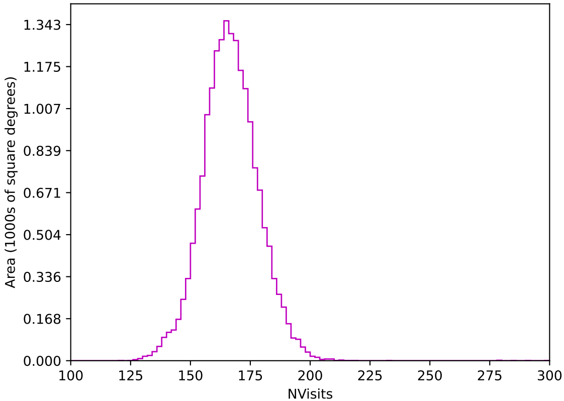
too_100_4v3.4_10yrs WFD z band: NVisits
