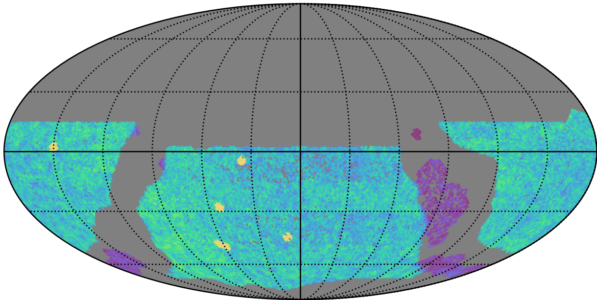
too_100_4v3.4_10yrs WFD u band: NVisits
