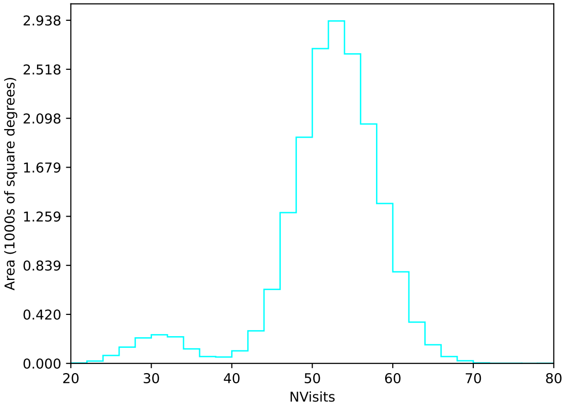
too_100_4v3.4_10yrs WFD u band: NVisits
