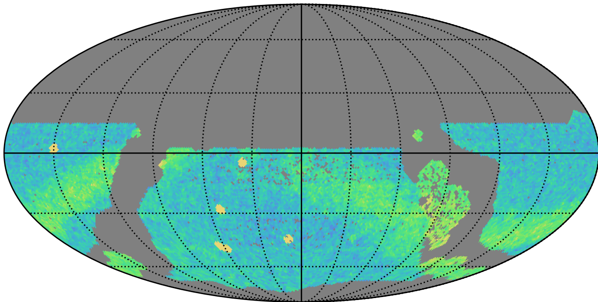
too_100_4v3.4_10yrs WFD r band: NVisits
