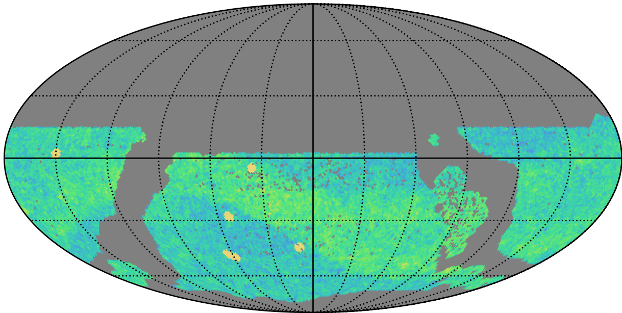
too_100_4v3.4_10yrs WFD i band: NVisits
