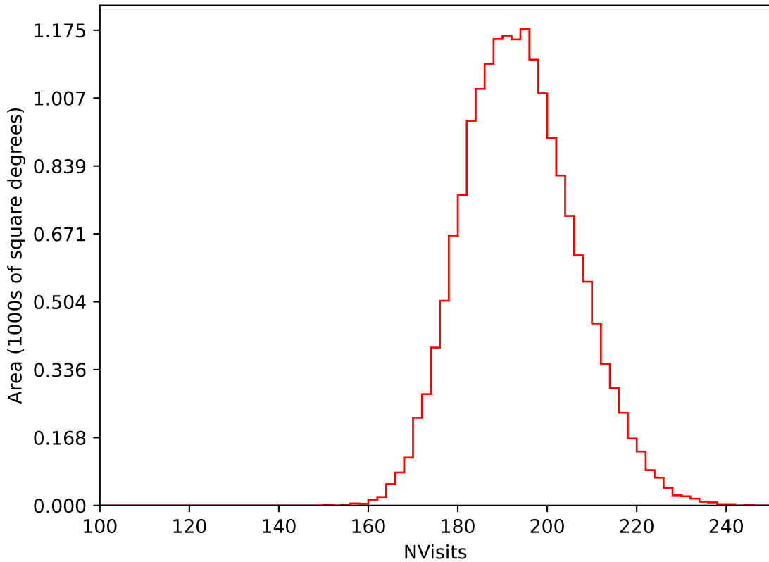
too_100_4v3.4_10yrs WFD i band: NVisits
