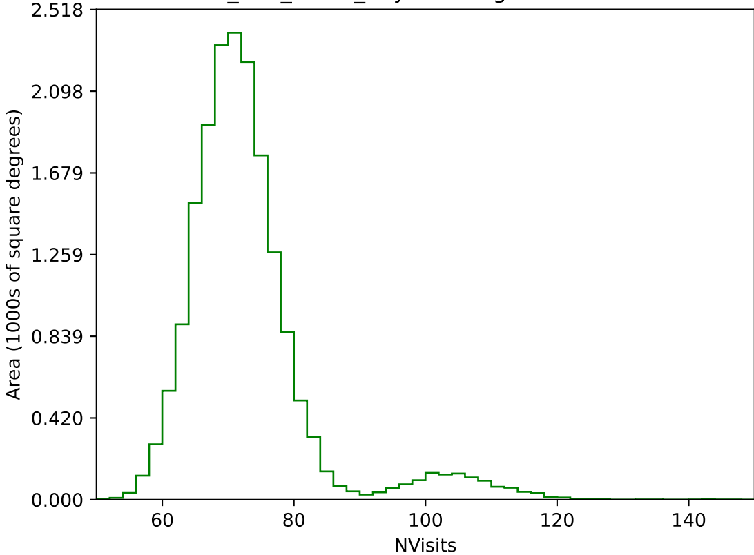
too_100_4v3.4_10yrs WFD g band: NVisits
