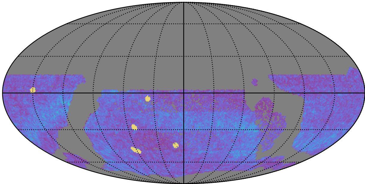
too_100_4v3.4_10yrs WFD all bands: NVisits
