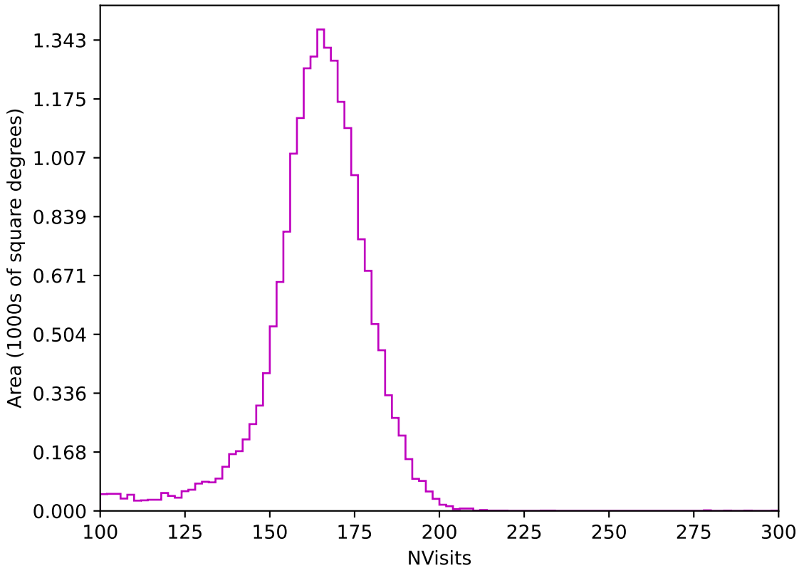
too_100_4v3.4_10yrs All sky z band: NVisits
