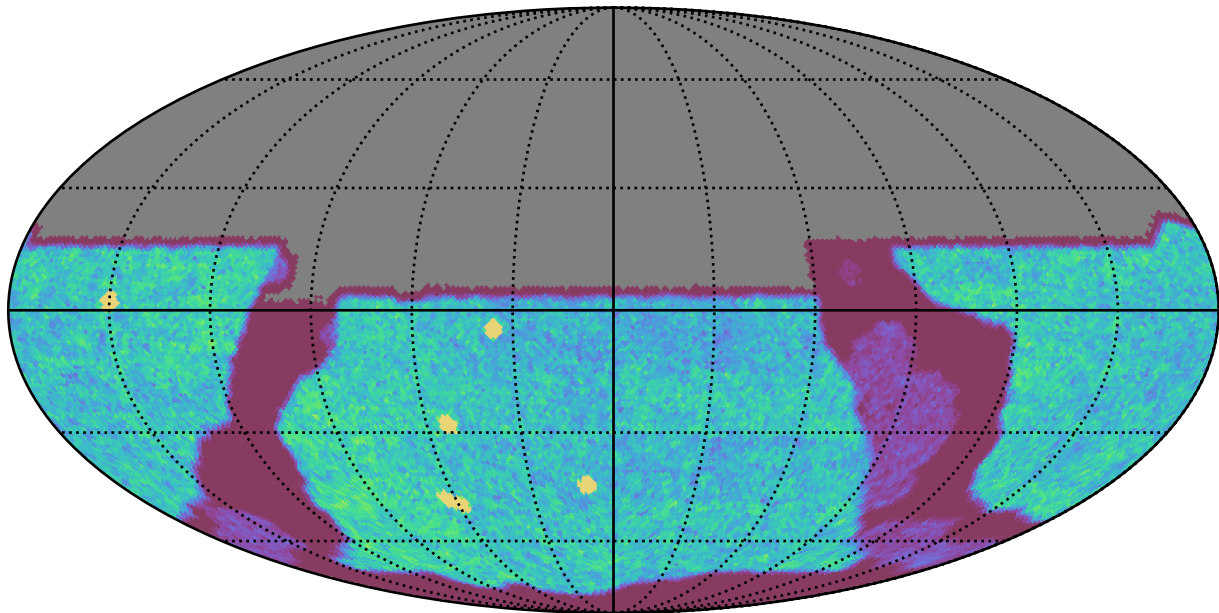
too_100_4v3.4_10yrs All sky u band: NVisits
