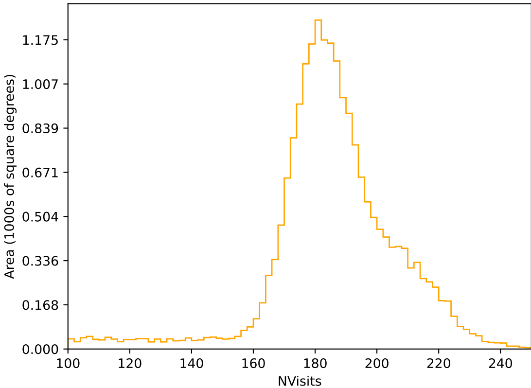
too_100_4v3.4_10yrs All sky r band: NVisits
