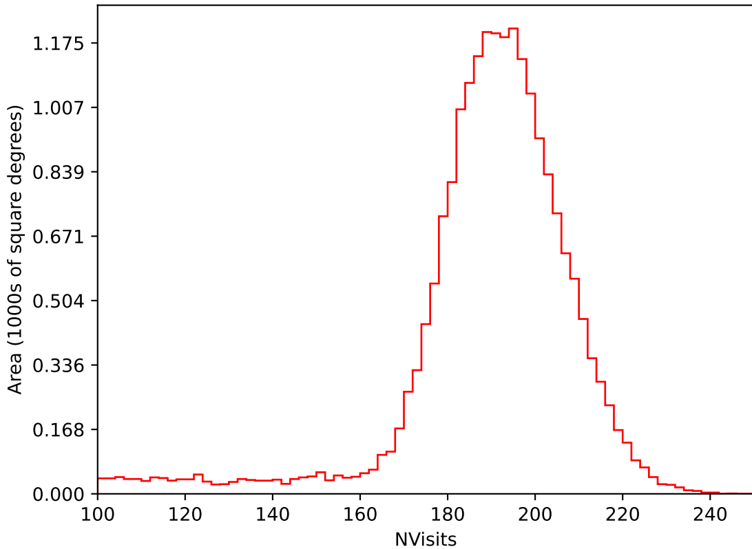
too_100_4v3.4_10yrs All sky i band: NVisits
