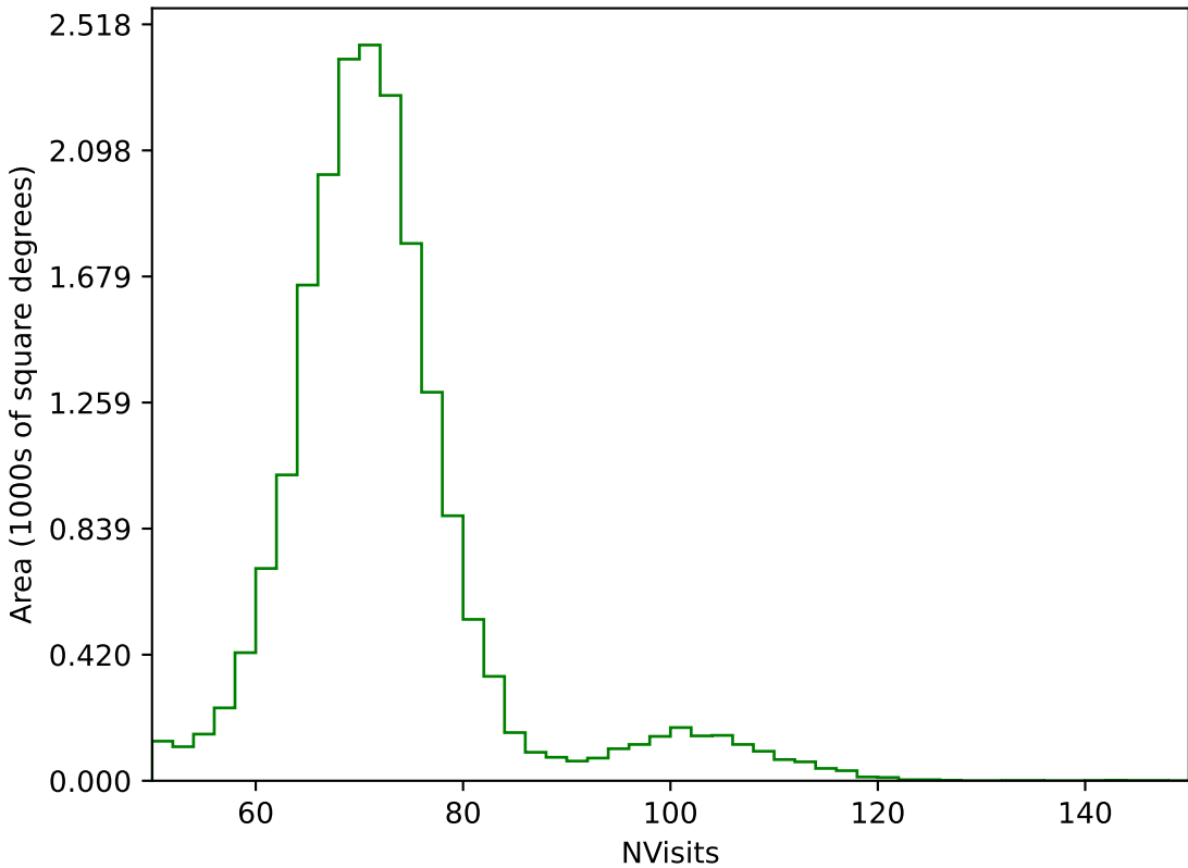
too_100_4v3.4_10yrs All sky g band: NVisits
