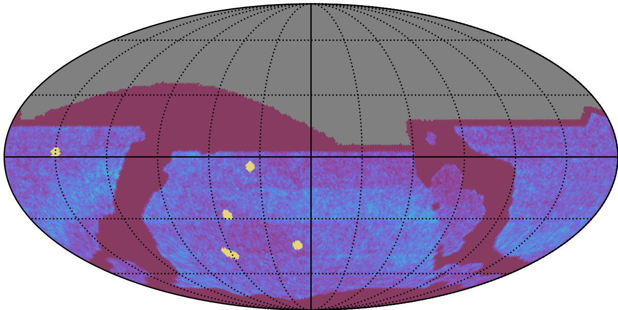
too_100_4v3.4_10yrs All sky all bands: NVisits
