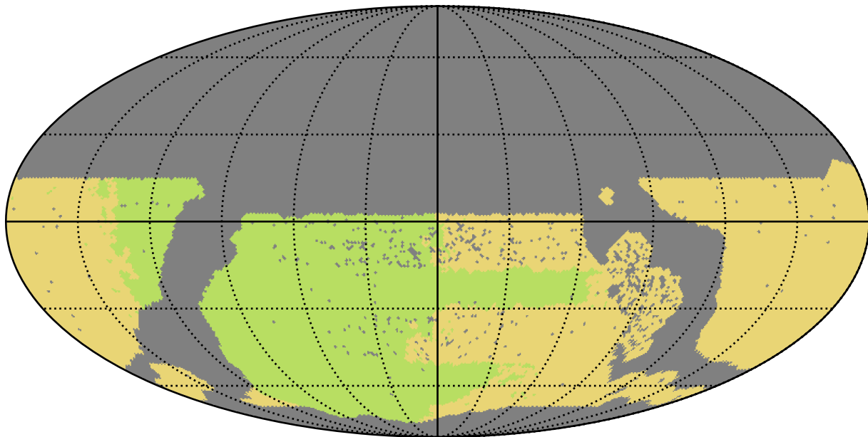
too_100_4v3.4_10yrs WFD all bands: NSeasons
