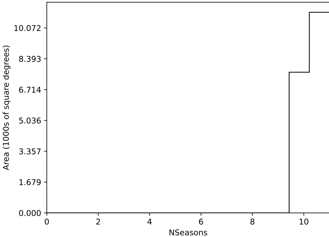
too_100_4v3.4_10yrs WFD all bands: NSeasons
