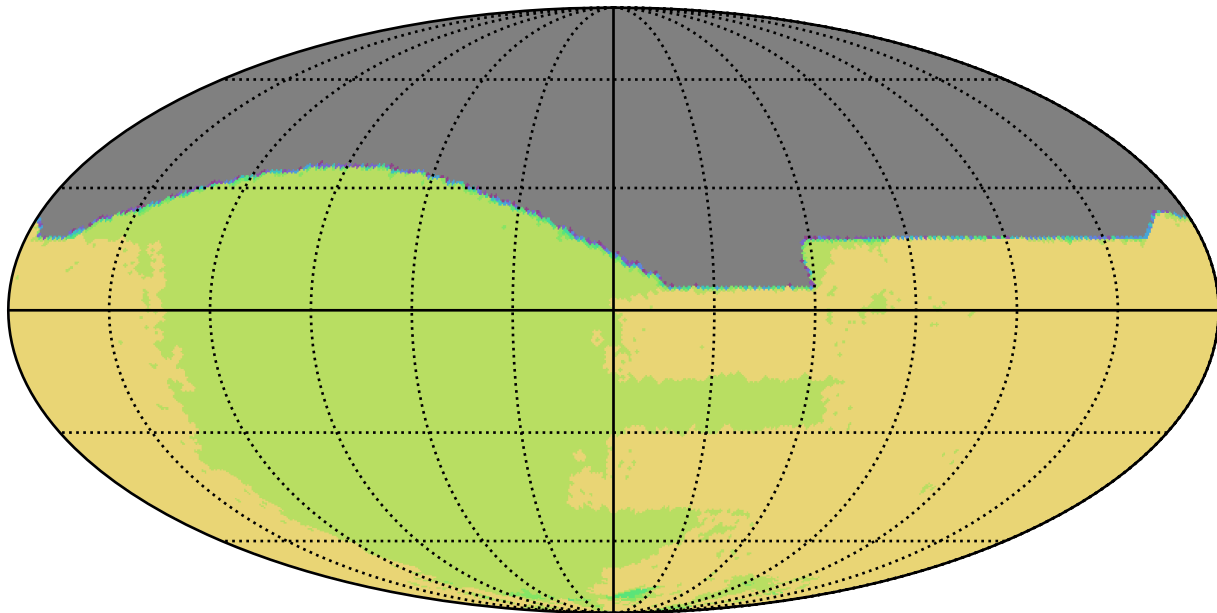
too_100_4v3.4_10yrs All sky all bands: NSeasons
