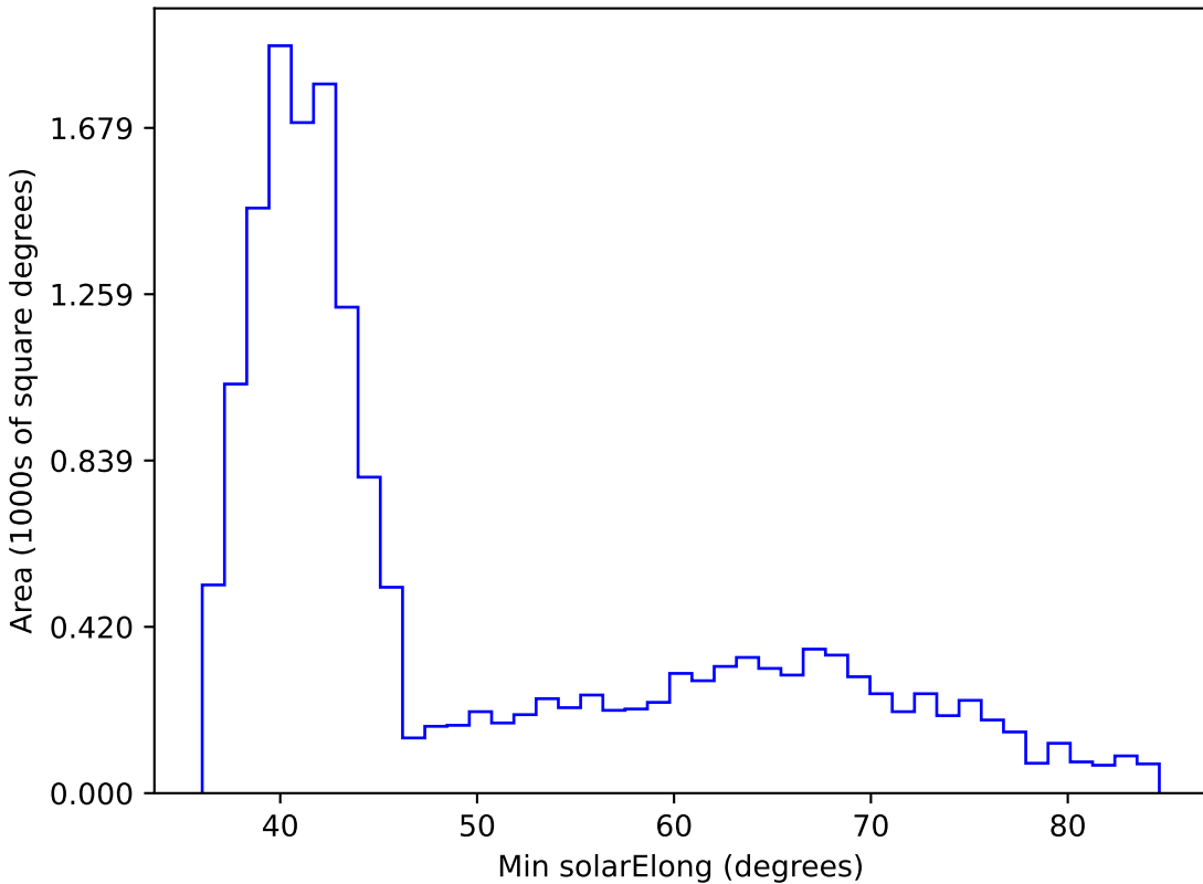
too_100_4v3.4_10yrs WFD z band: Min solarElong
