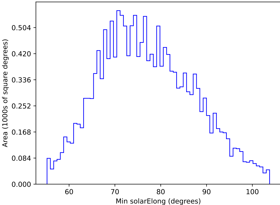
too_100_4v3.4_10yrs WFD u band: Min solarElong
