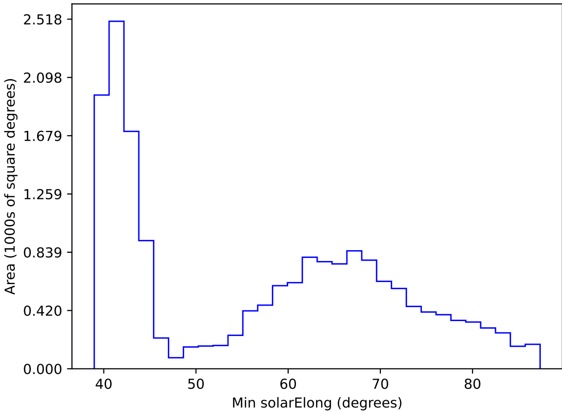
too_100_4v3.4_10yrs WFD r band: Min solarElong
