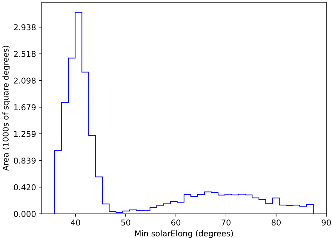
too_100_4v3.4_10yrs WFD i band: Min solarElong
