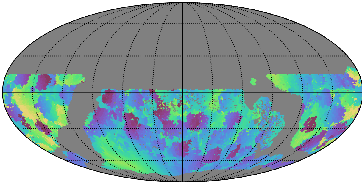
too_100_4v3.4_10yrs WFD g band: Min solarElong
