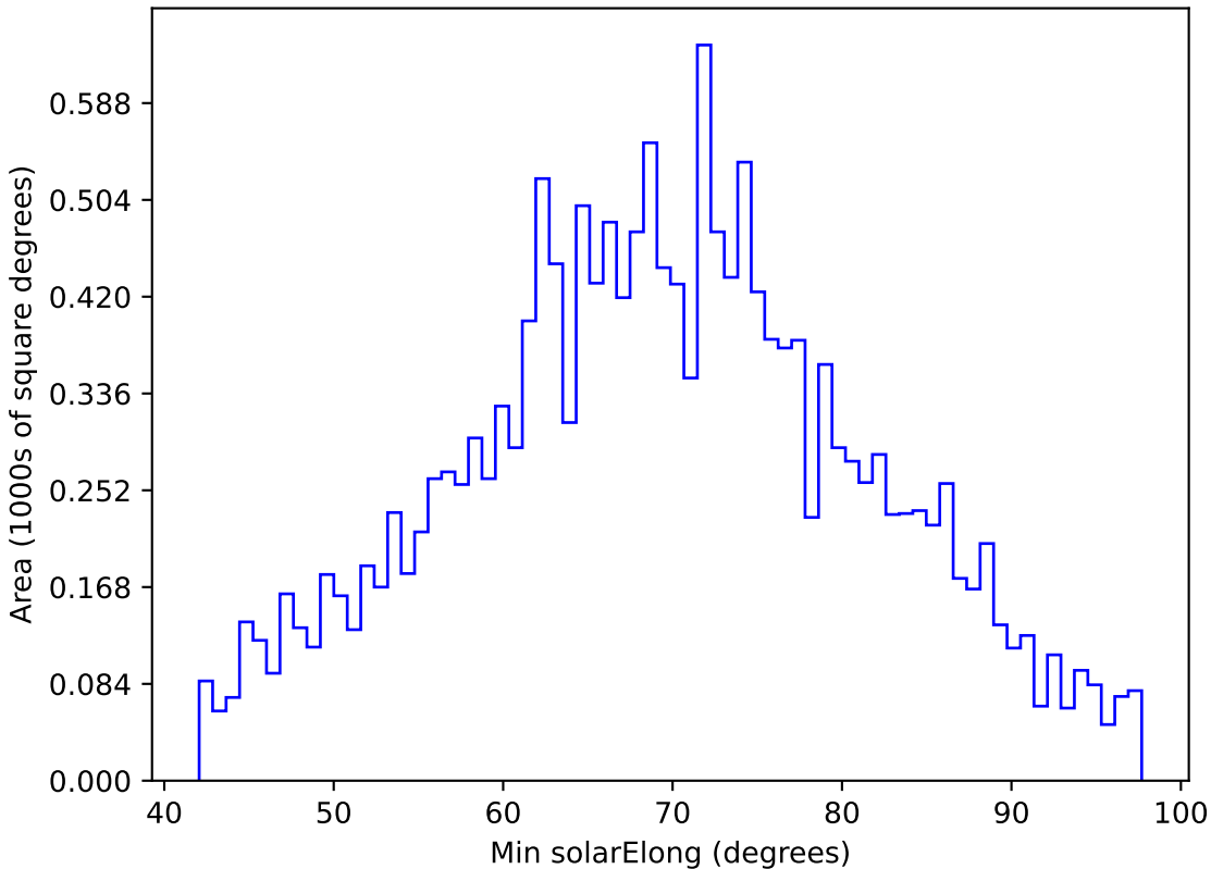
too_100_4v3.4_10yrs WFD g band: Min solarElong
