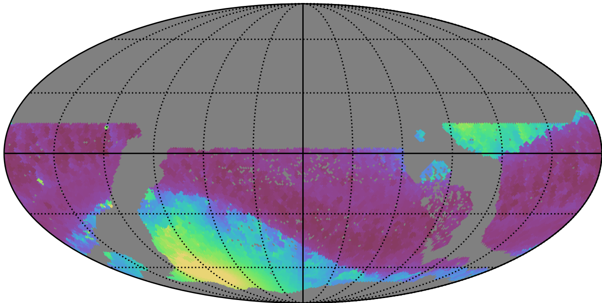
too_100_4v3.4_10yrs WFD all bands: Min solarElong
