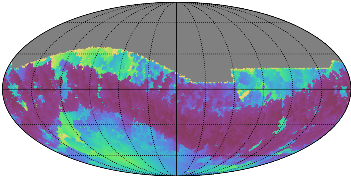
too_100_4v3.4_10yrs All sky z band: Min solarElong
