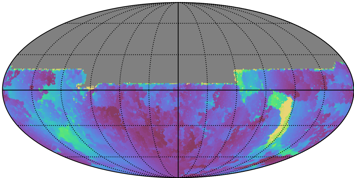
too_100_4v3.4_10yrs All sky u band: Min solarElong
