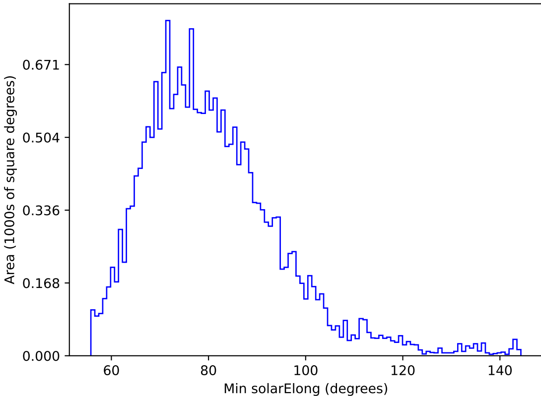
too_100_4v3.4_10yrs All sky u band: Min solarElong
