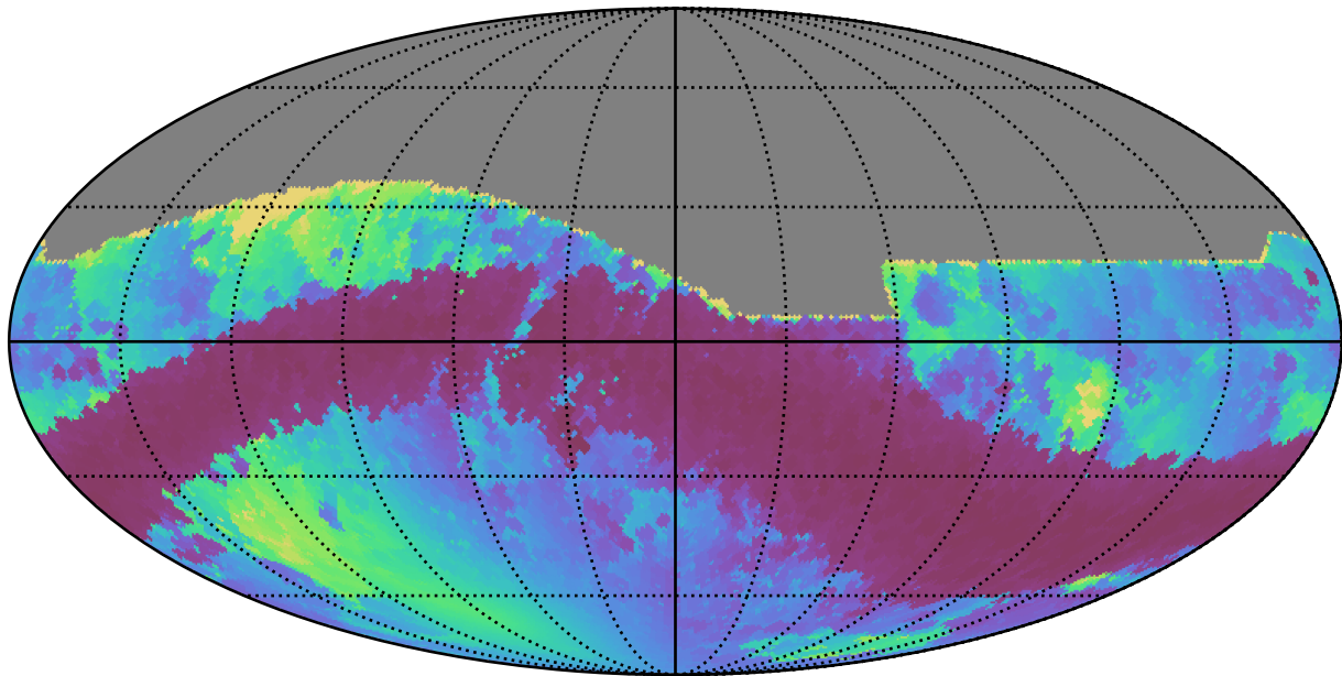
too_100_4v3.4_10yrs All sky r band: Min solarElong
