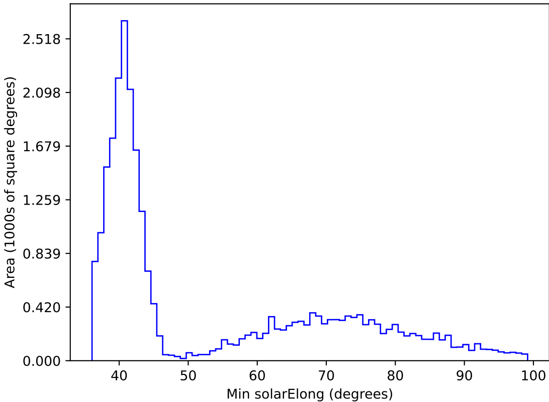
too_100_4v3.4_10yrs All sky i band: Min solarElong
