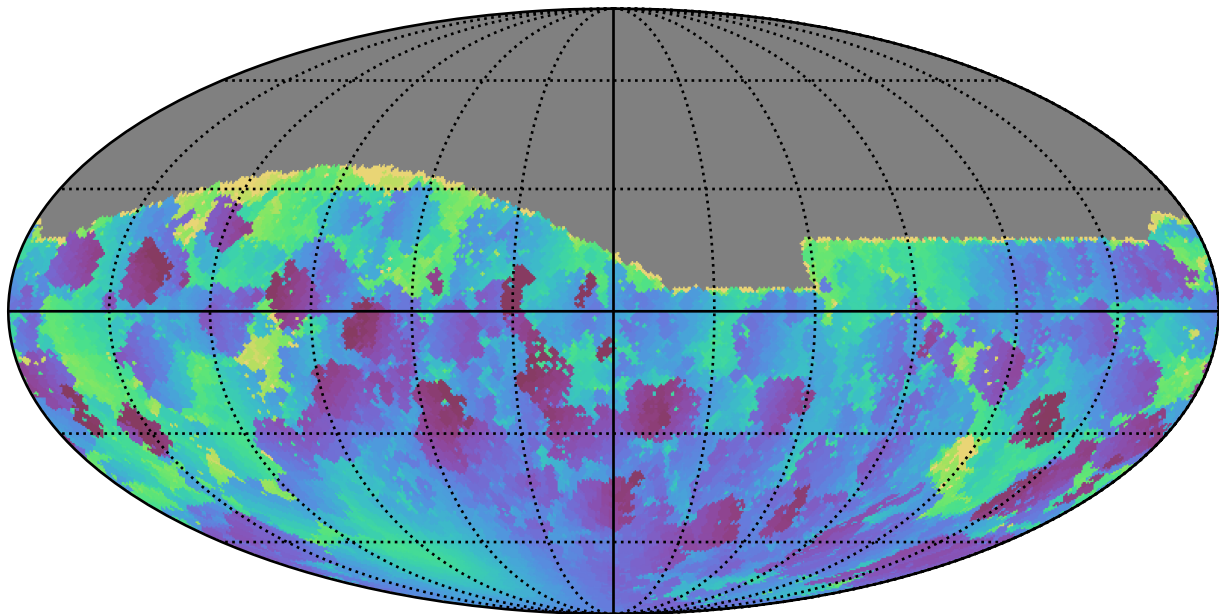
too_100_4v3.4_10yrs All sky g band: Min solarElong
