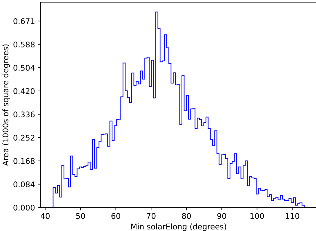
too_100_4v3.4_10yrs All sky g band: Min solarElong
