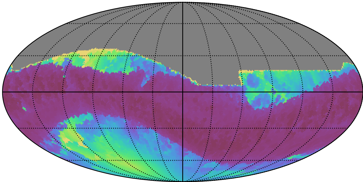
too_100_4v3.4_10yrs All sky all bands: Min solarElong
