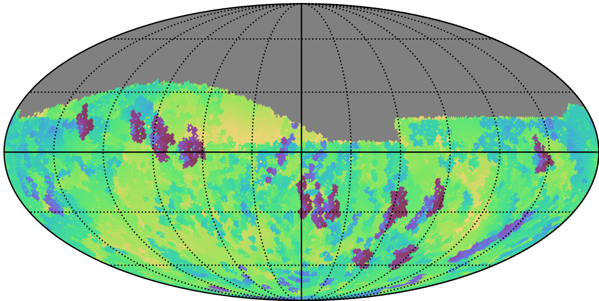
too_100_4v3.4_10yrs Yr 1 z band: Min skyBrightness
