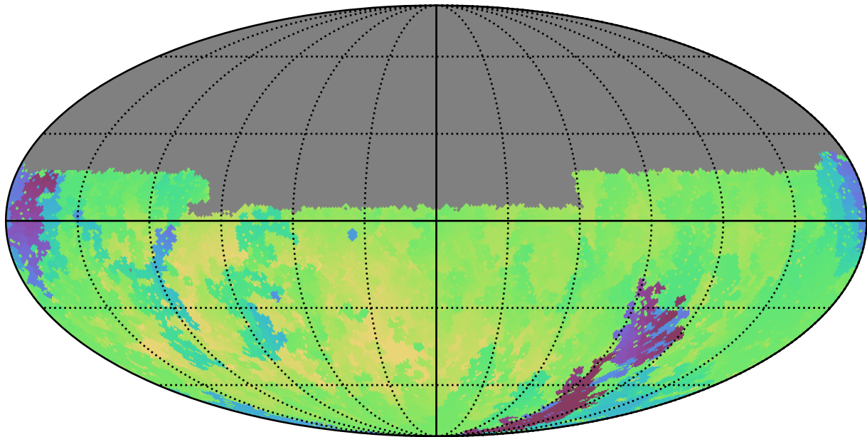
too_100_4v3.4_10yrs Yr 1 u band: Min skyBrightness
