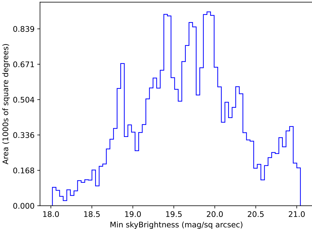
too_100_4v3.4_10yrs Yr 1 r band: Min skyBrightness
