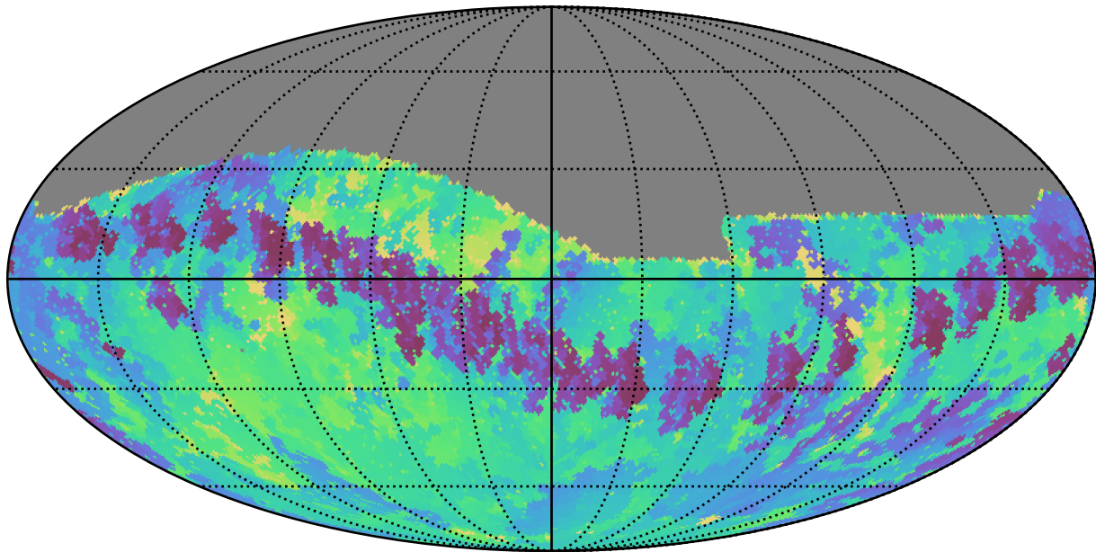
too_100_4v3.4_10yrs Yr 1 i band: Min skyBrightness
