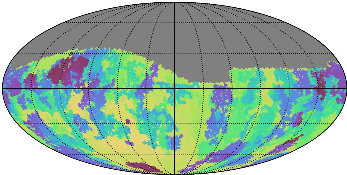
too_100_4v3.4_10yrs Yr 1 g band: Min skyBrightness
