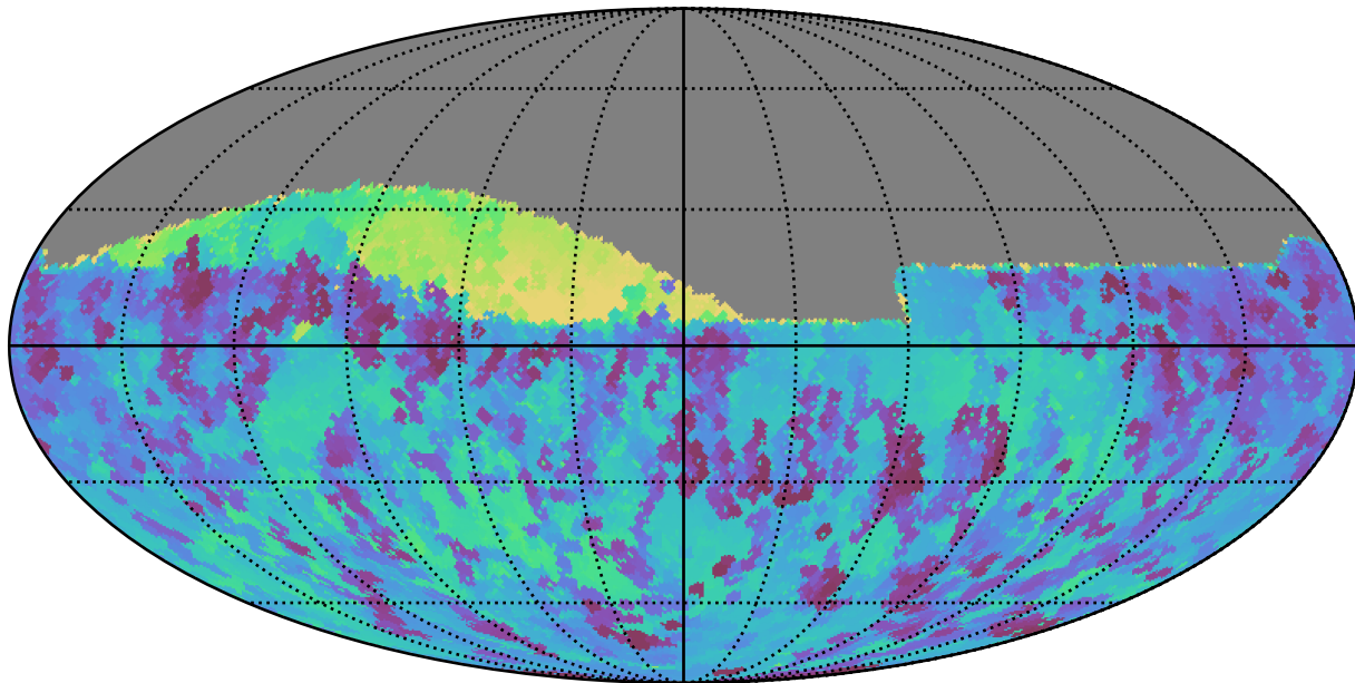
too_100_4v3.4_10yrs Yr 1 all bands: Min skyBrightness
