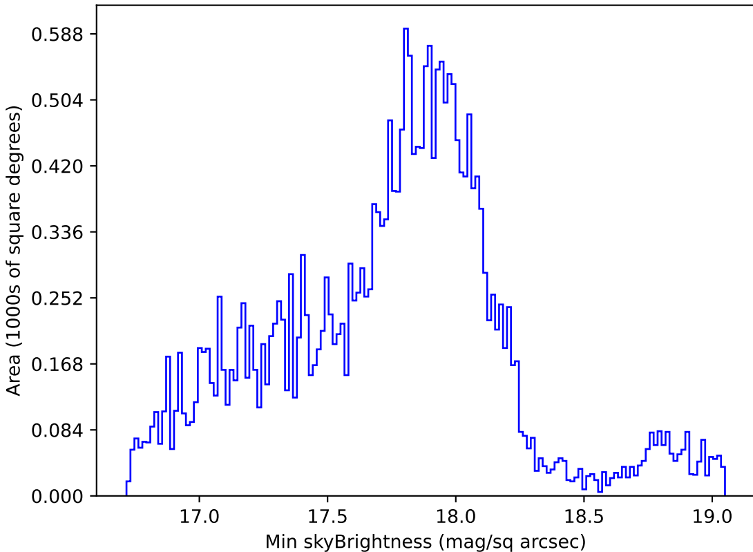
too_100_4v3.4_10yrs Yr 1 all bands: Min skyBrightness
