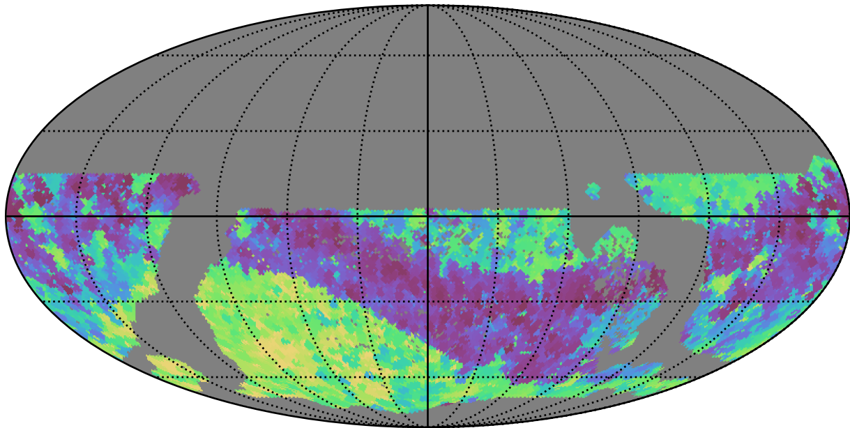
too_100_4v3.4_10yrs WFD z band: Min skyBrightness
