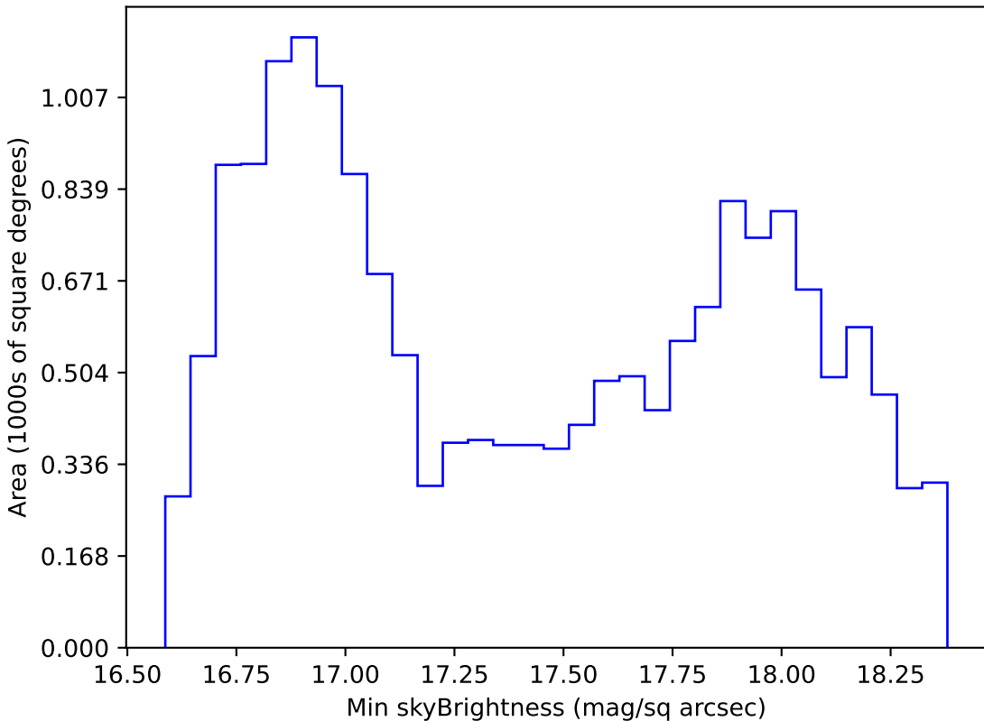
too_100_4v3.4_10yrs WFD z band: Min skyBrightness
