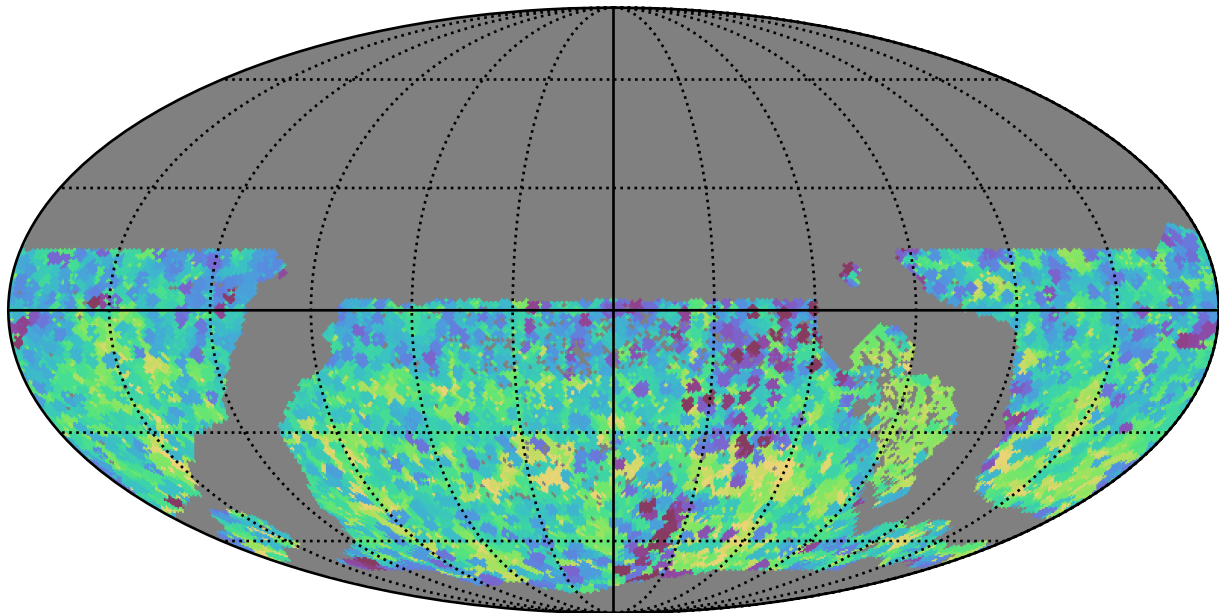
too_100_4v3.4_10yrs WFD y band: Min skyBrightness
