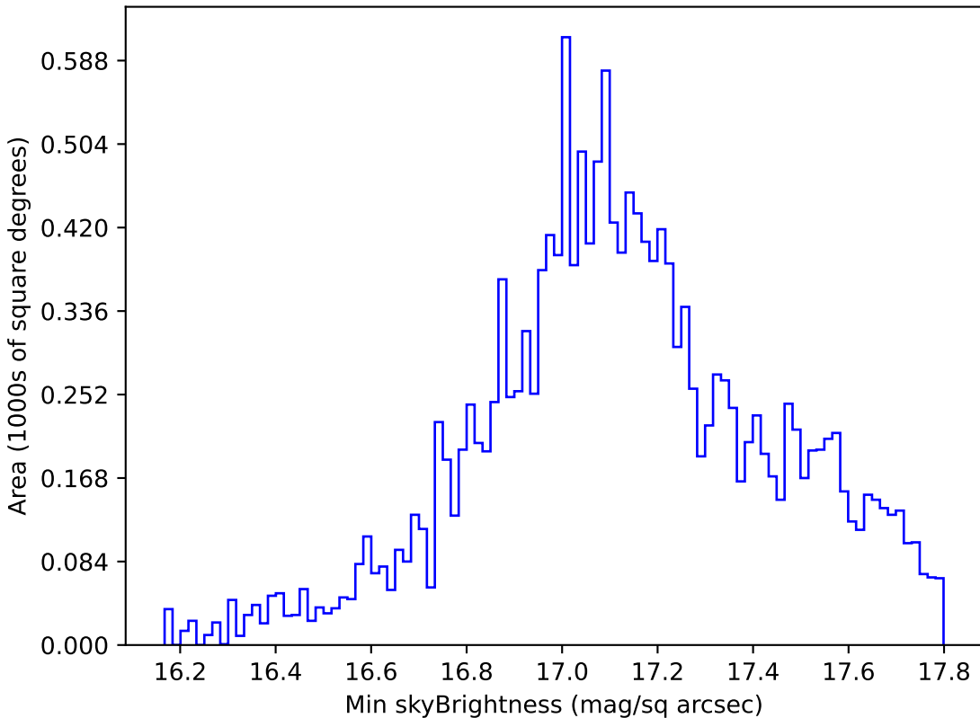
too_100_4v3.4_10yrs WFD y band: Min skyBrightness
