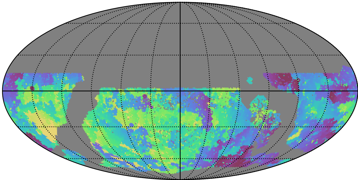
too_100_4v3.4_10yrs WFD u band: Min skyBrightness
