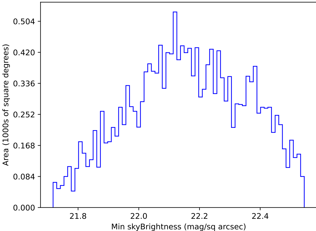
too_100_4v3.4_10yrs WFD u band: Min skyBrightness
